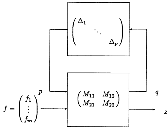
Fig. 1. Setup for robust \mathcal{H}_2 analysis.
